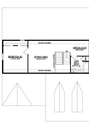
LAUREL 2ND FLOOR PLAN RE27
