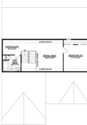
LAUREL 2ND FLOOR PLAN RE28
