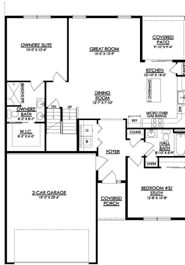
LAUREL 1ST FLOOR PLAN RE28
