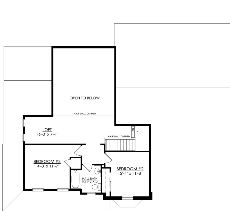
MARELLA STARTING AT 2540 SF 2ND FLOOR PLAN
