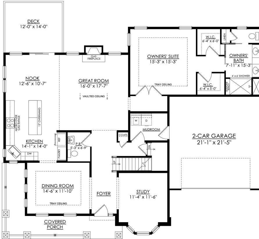
MARELLA STARTING AT 2540 SF 1ST FLOOR PLAN
