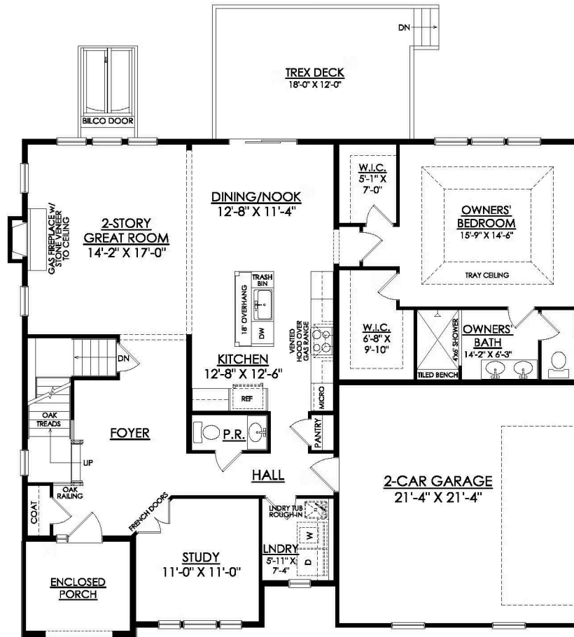
VINECREST COTTAGE 1ST FLOOR PLAN ESTATES AT STEEPLECHASE NORTH-
