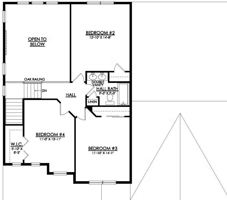
VINECREST TRADITIONAL 2ND FLOOR PLAN SC113
