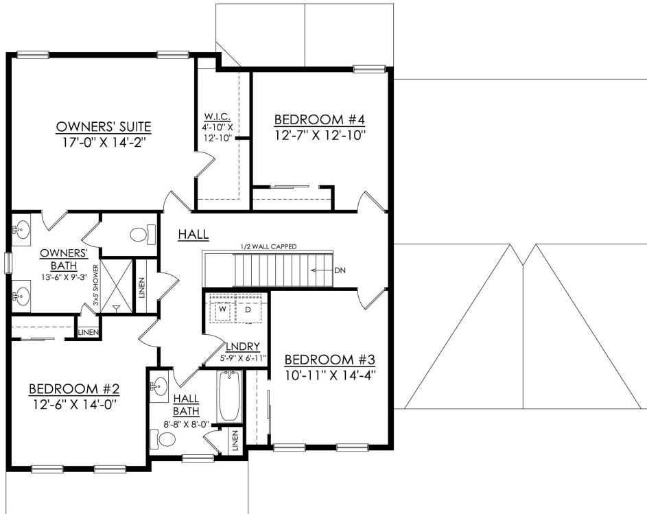
MERIDIAN CRAFTSMAN STARTING AT 2848 SF
