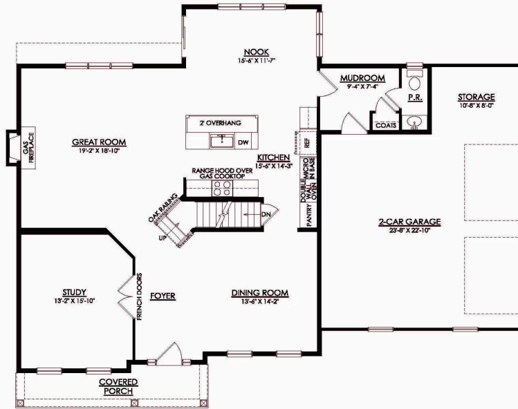
MAGNOLIA CRAFTSMAN 1ST FLOOR PLAN
