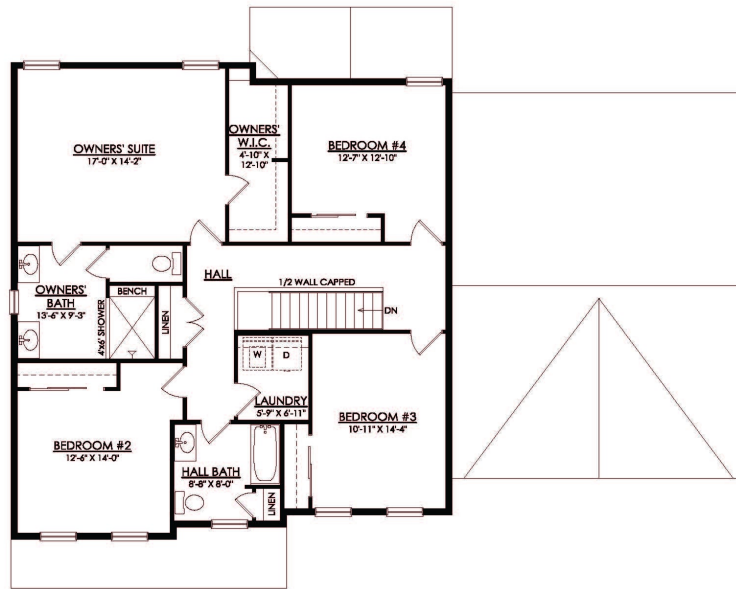
MERIDIAN CRAFTSMAN 2ND FLOOR PLAN
