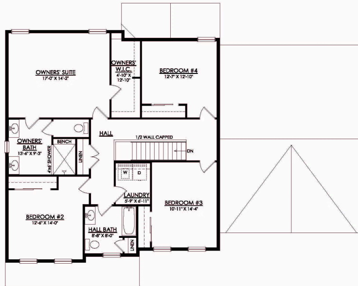
MAGNOLIA CRAFTSMAN 2ND FLOOR PLAN
