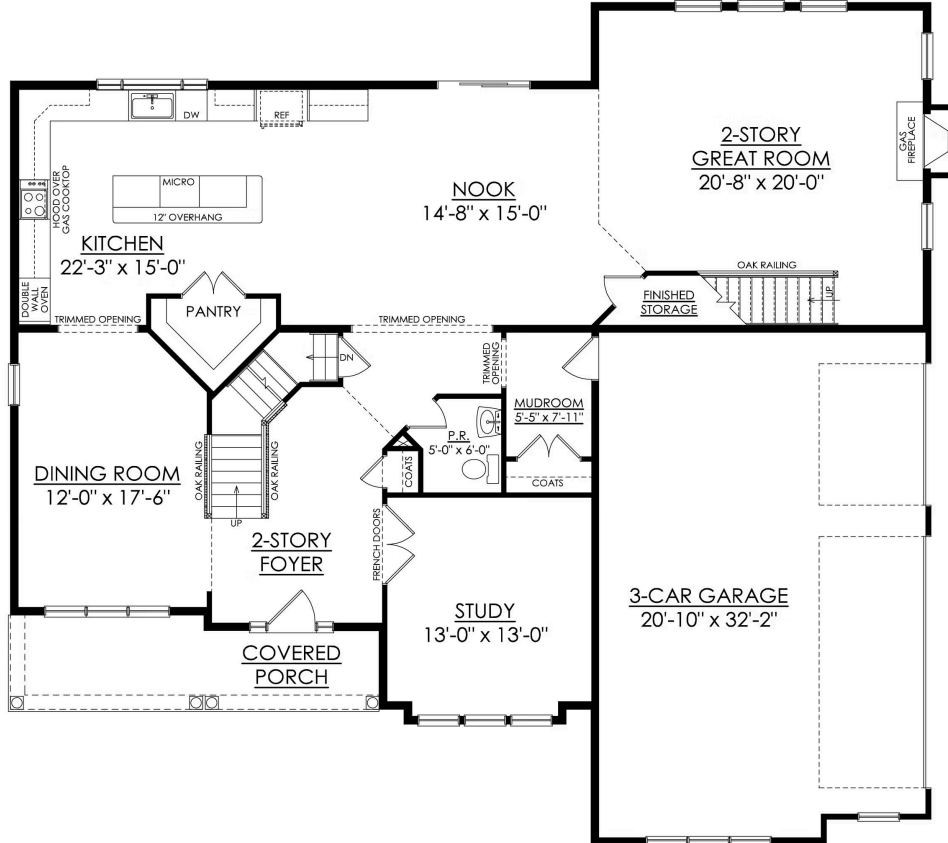
PREAKNESS FARMHOUSE 1ST FLOOR PLAN OPTION #00509- PREAKNESS GOURMET KITCHEN
