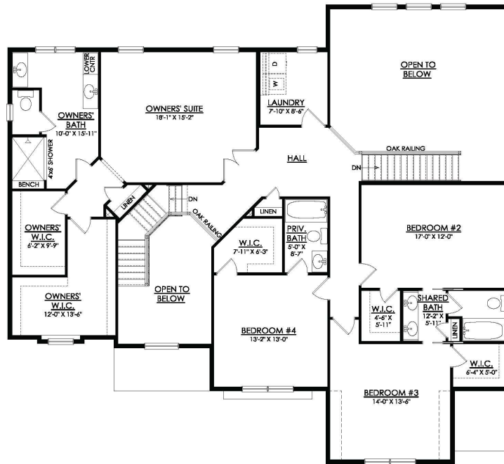
PREAKNESS TRADITIONAL 2ND FLOOR PLAN
