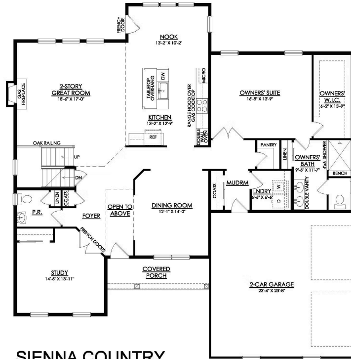
SIENNA COUNTRY 1ST FLOOR PLAN
