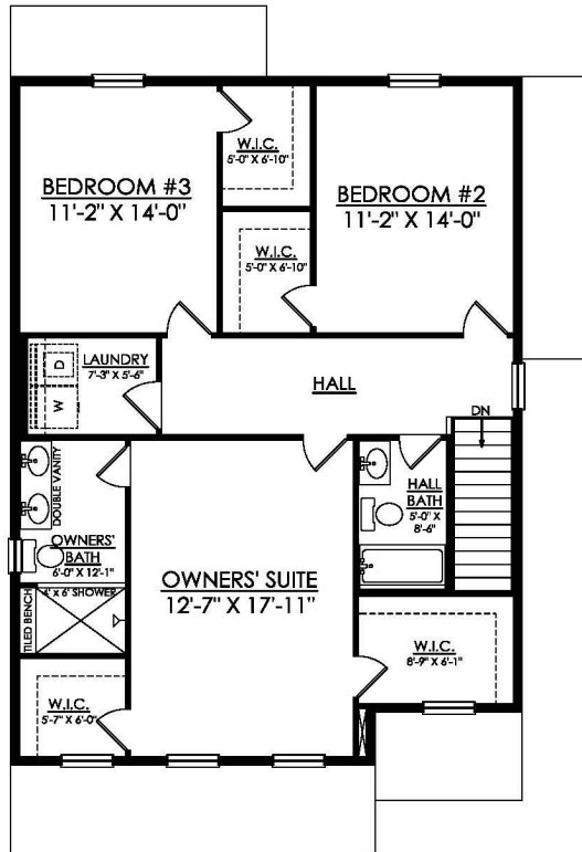
MIA HILLCREST ESTATES LOT #72 2ND FLOOR PLAN 1106 SF
